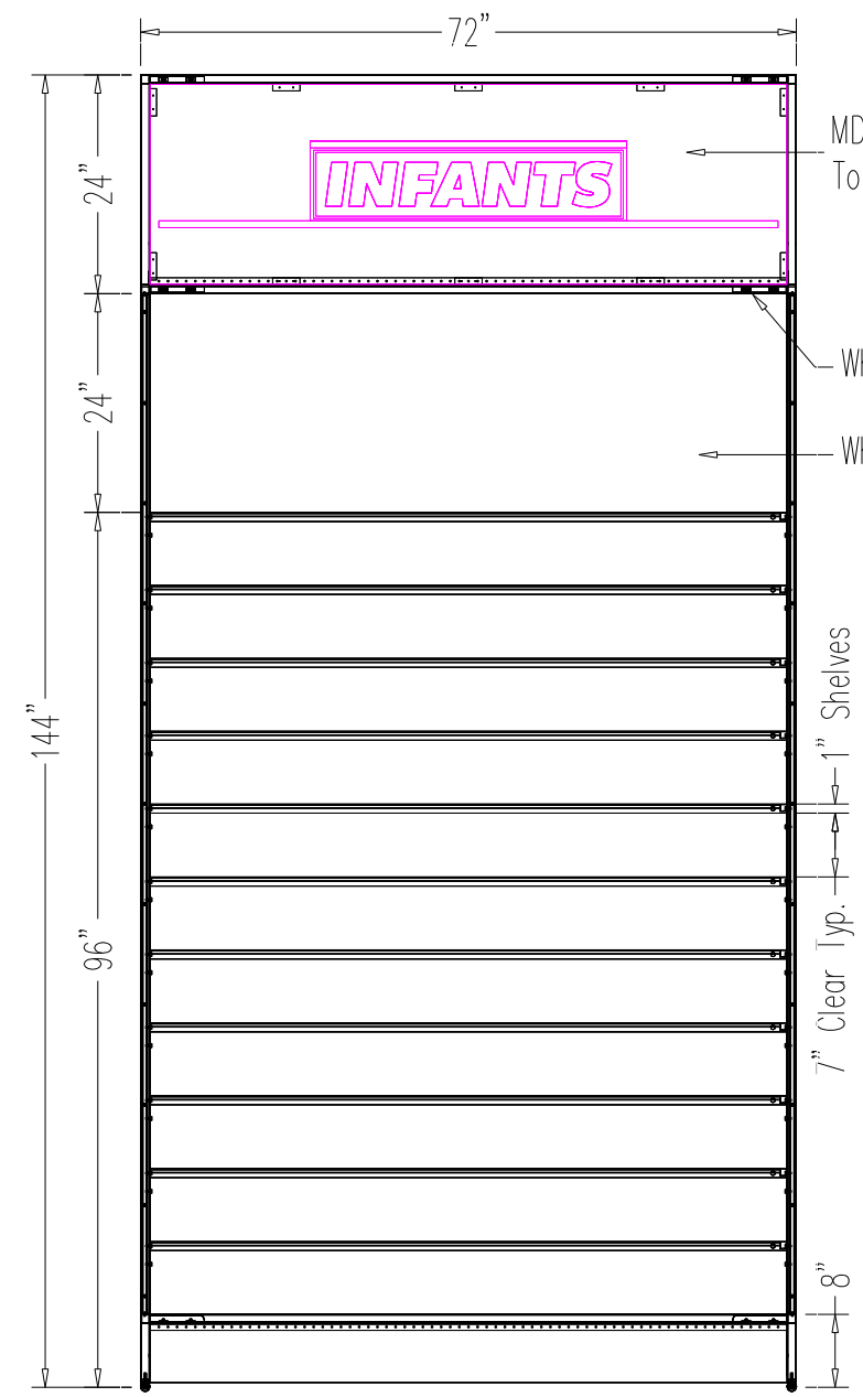
Front No Scale
