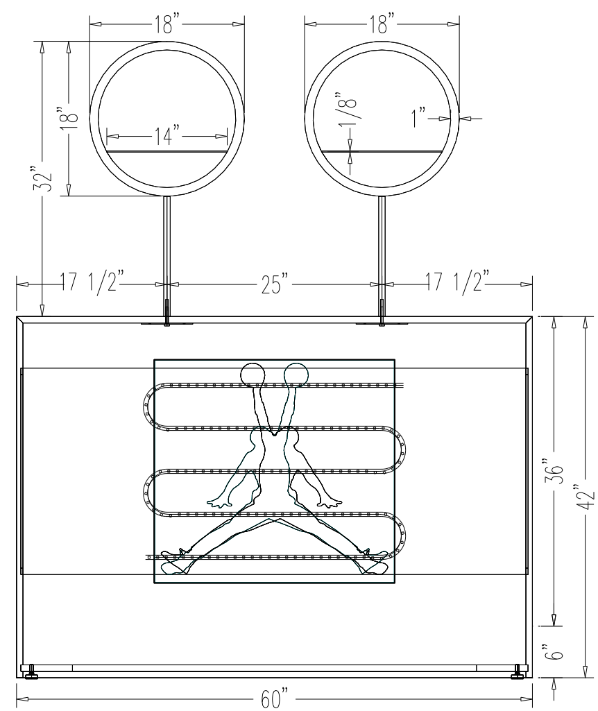
Elevation No Scale
