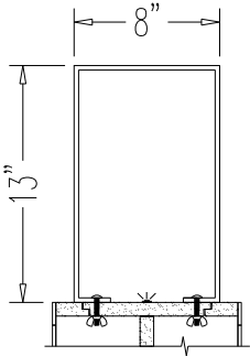
End Section No Scale
