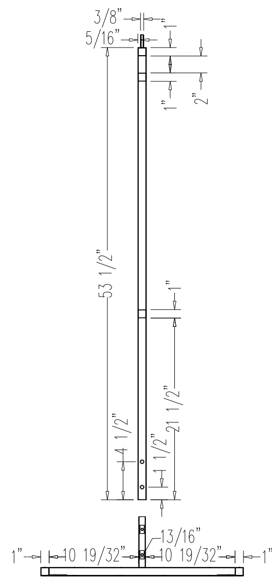
End Section No Scale
