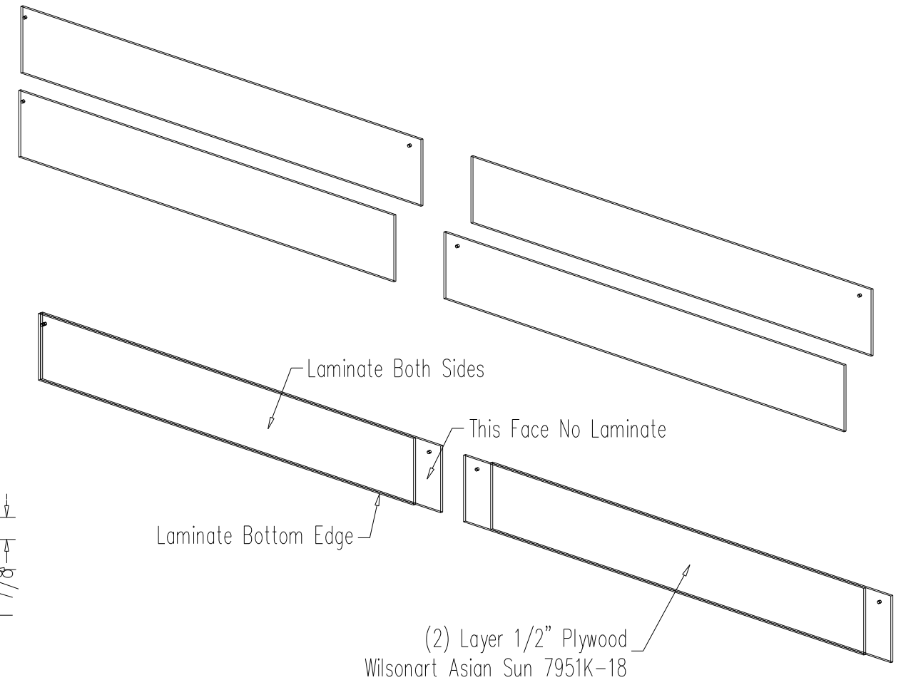
Perspective No Scale
