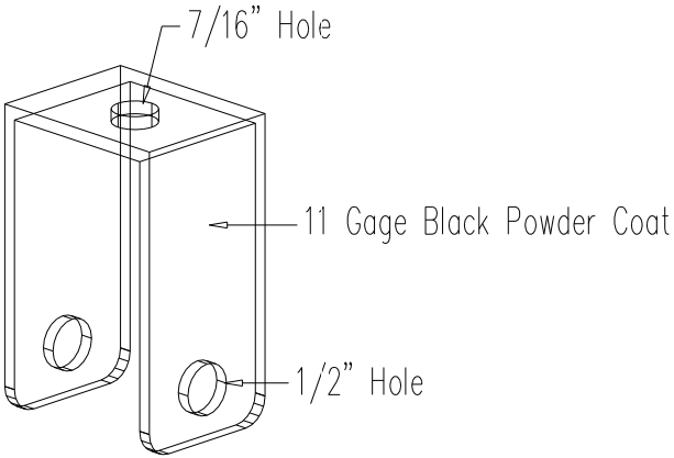
Perspective No Scale
