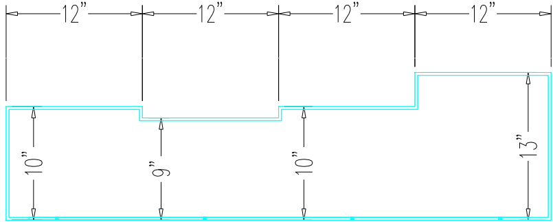
Side No Scale
