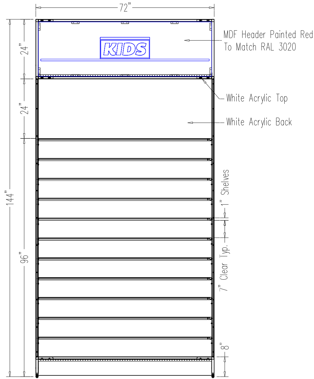
Front No Scale
