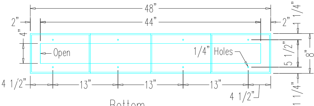
Bottom No Scale
