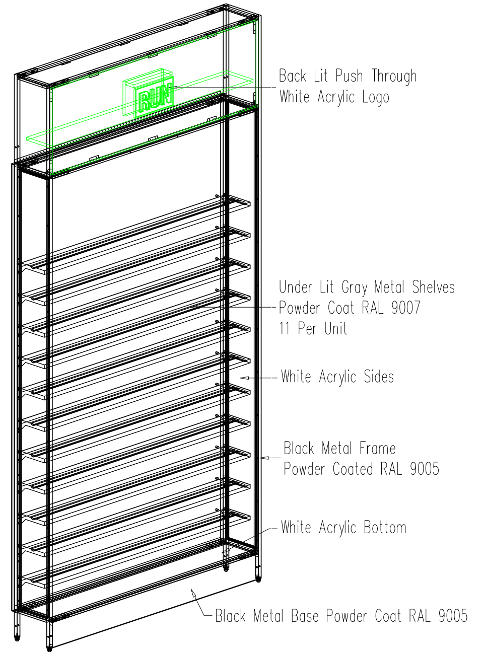
Perspective No Scale
