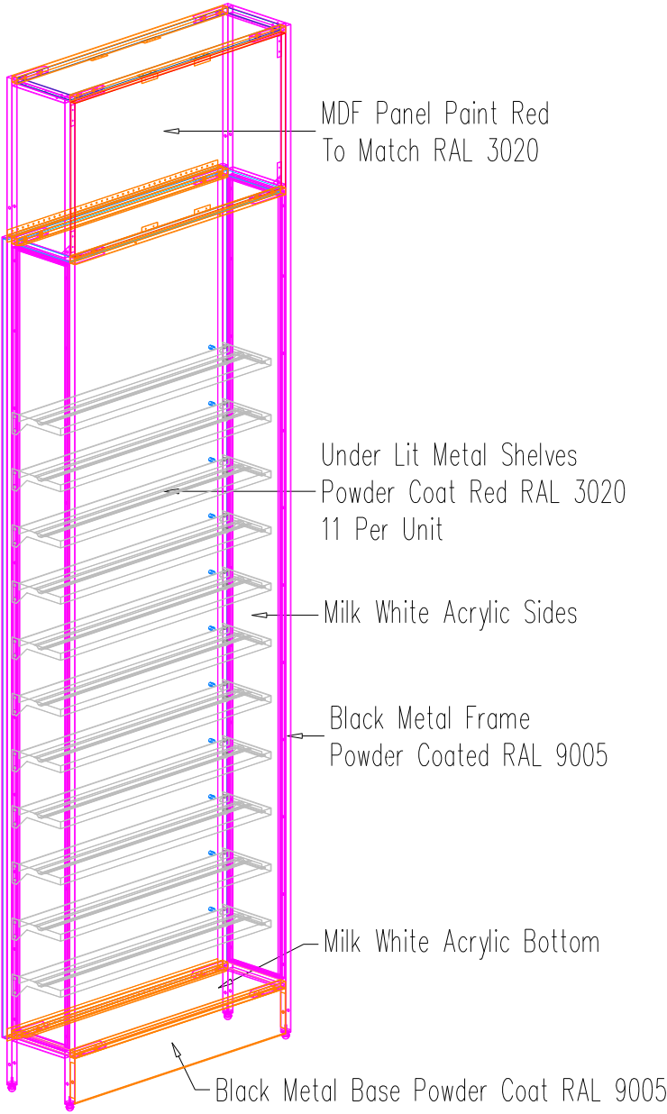
Perspective No Scale
