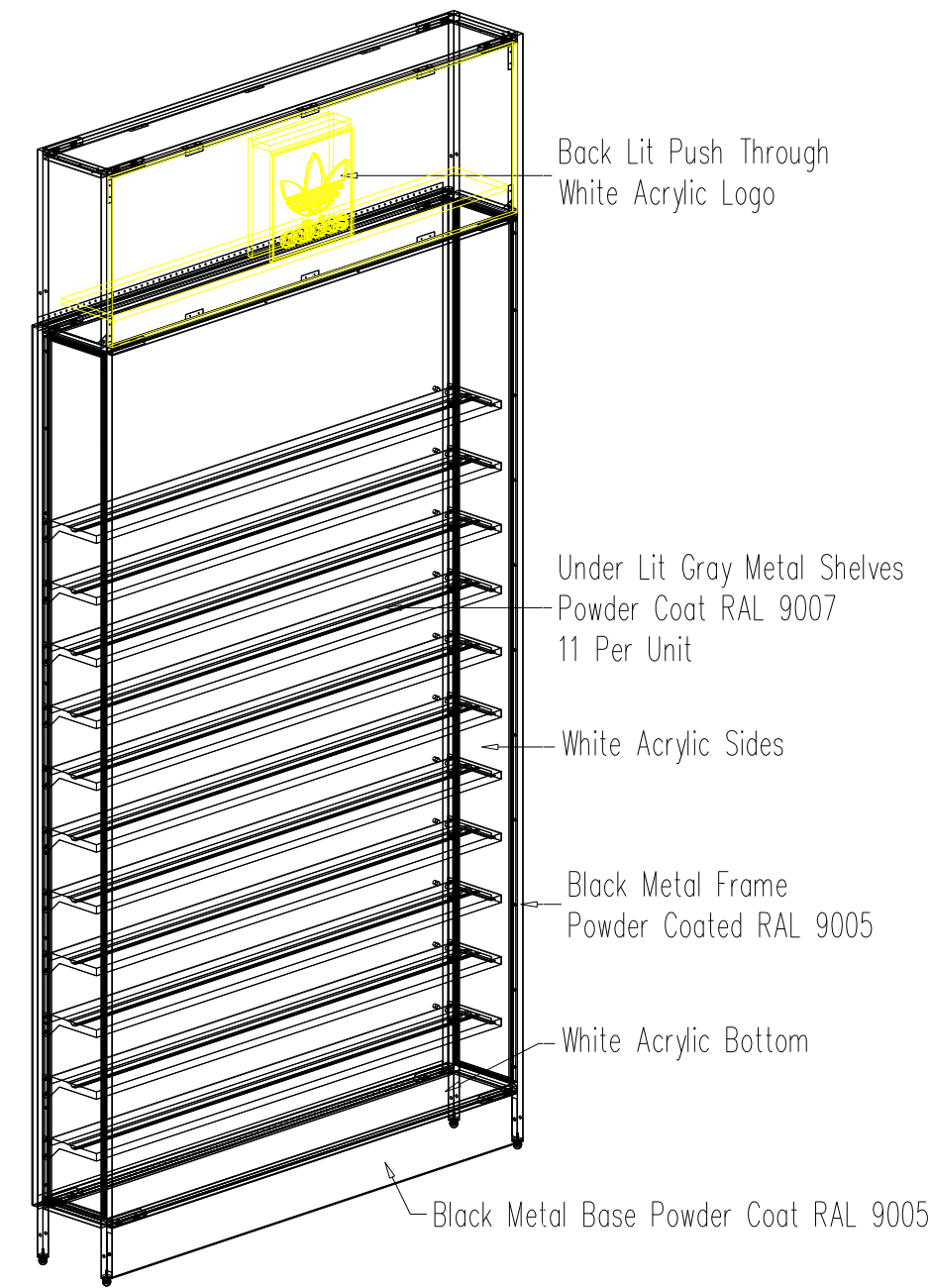
Perspective No Scale
