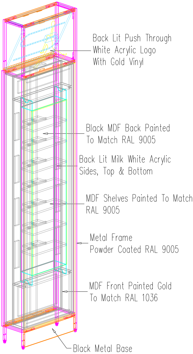
Perspective No Scale
