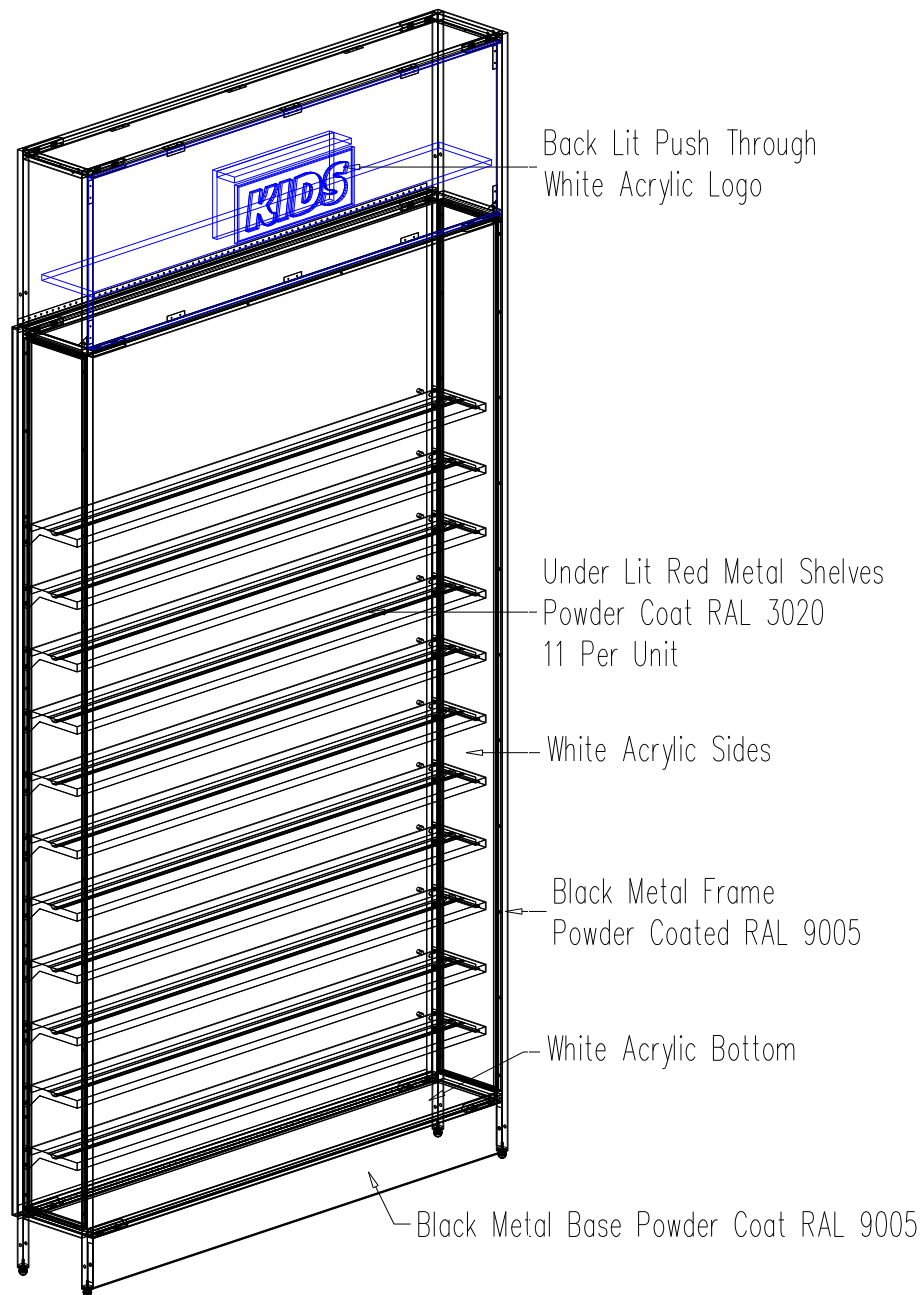
Perspective No Scale
