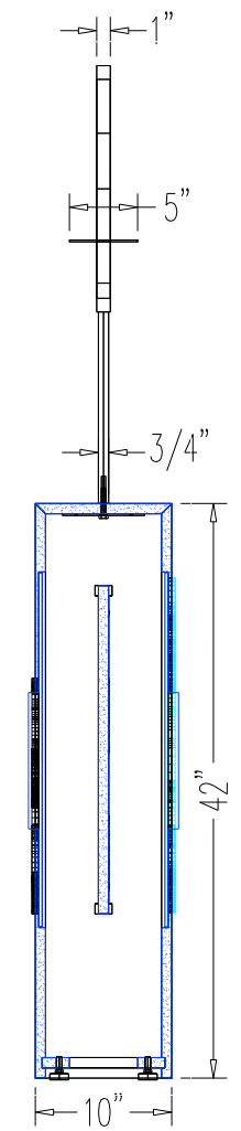
End Section No Scale
