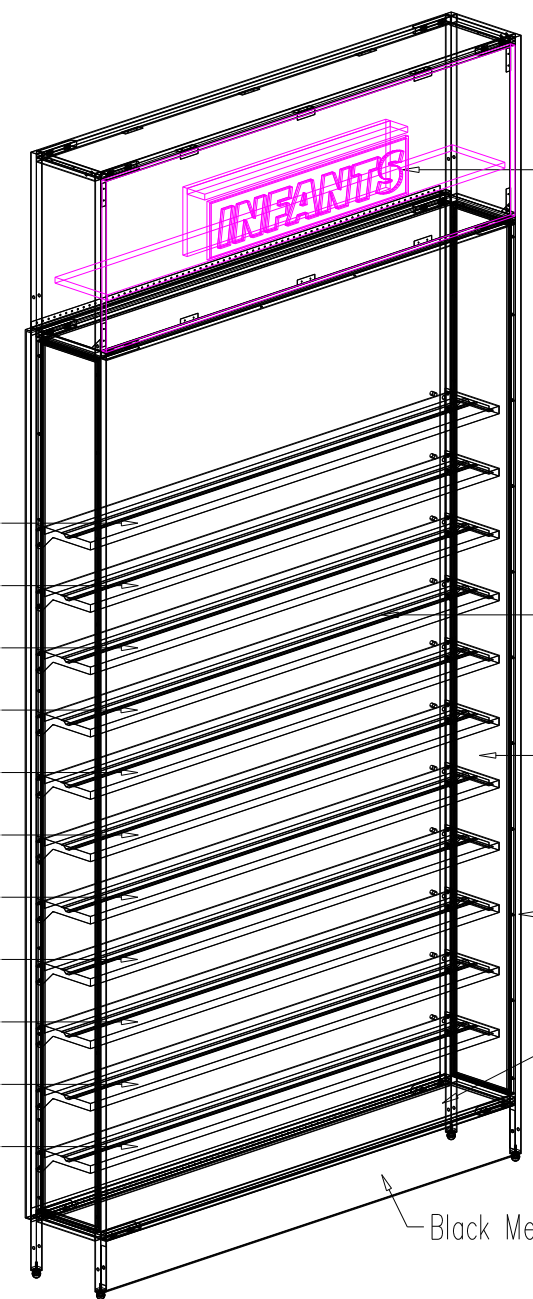
Perspective No Scale
