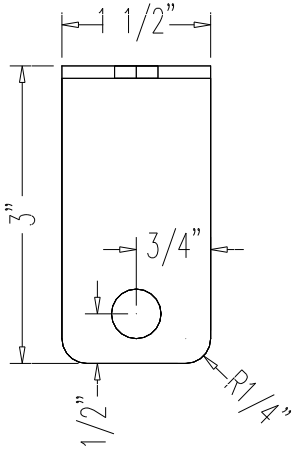
Side No Scale
