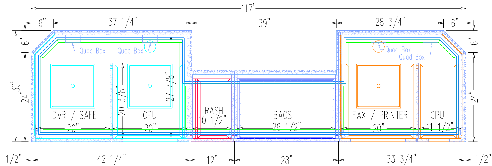
Plan Section Bottom No Scale
